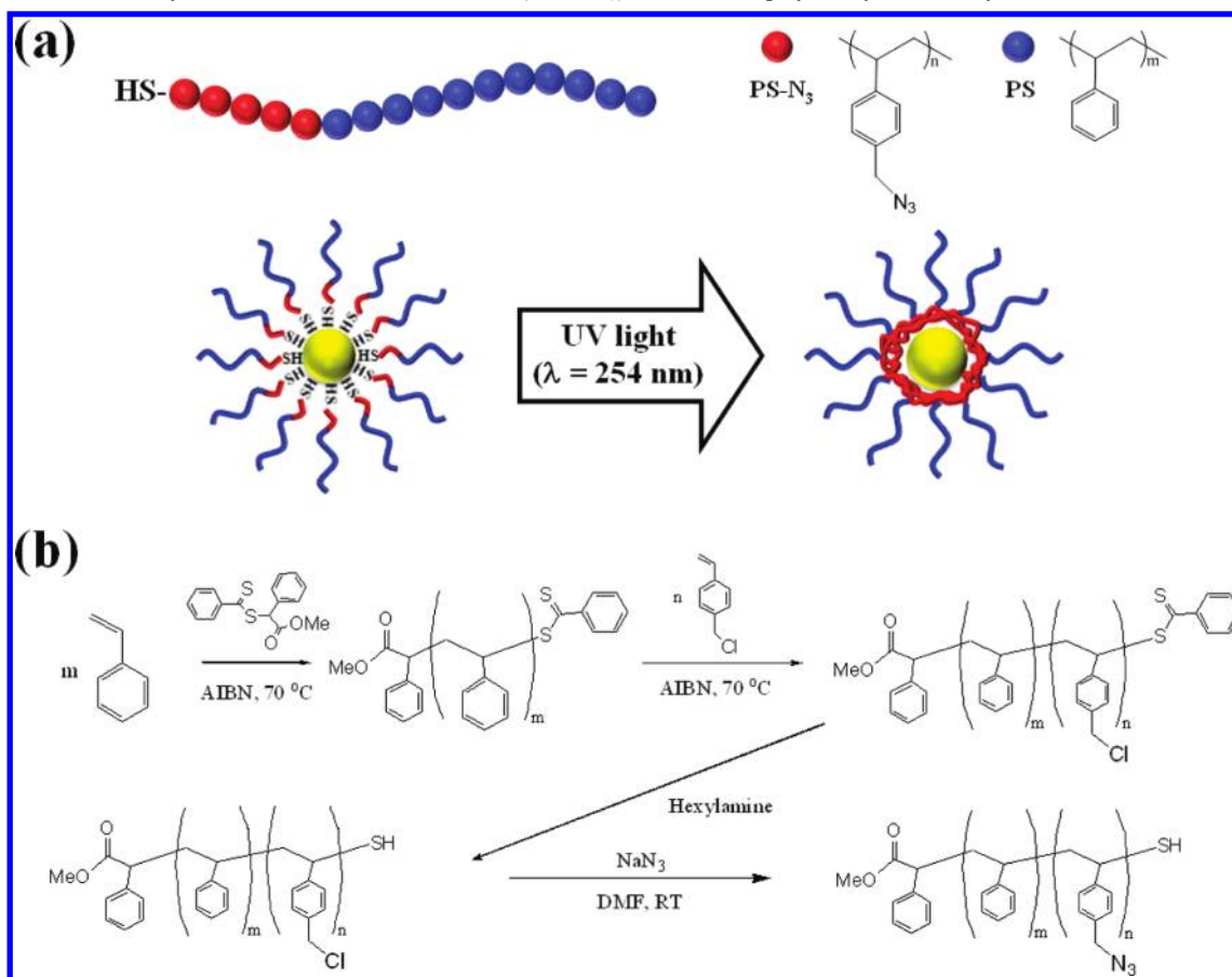
Scheme 1. Schematic Illustration for (a) the Design of Shell-Protected Au NPs via UV Cross-Linking Reaction of Azido ( -N_3 ) Group and (b) the Synthesis of Photo-Cross-Linkable P(S- b -S- N_3 )-SH Block Copolymer by RAFT Polymerization
