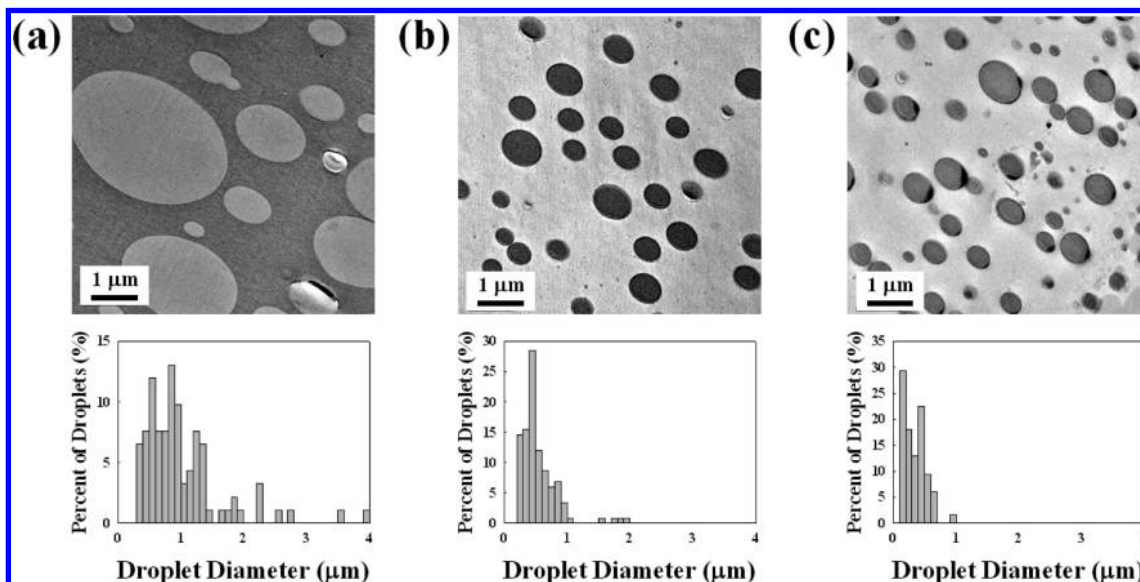
Figure 4. TEM images and the corresponding droplet size distribution of PS/PMMA(50:50) blends with cross-linked Au NPs as compatibilizer, after annealing at 180 °C for 48 h. The amounts of cross-linked Au NPs in blends are (a) 0.0, (b) 5.0, and (c) 10.0 wt %.
